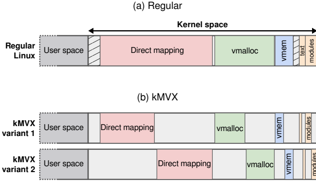
Figure 3: Regular kernel virtual address space, and the kMVX partitioned non-overlapping address space.
