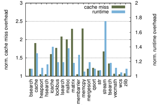
Figure 5: stress-ng. We measure the performance of kMVX on userspace benchmarks making use of few syscalls. We show how cache performance is affected by kMVX. stress-ng is configured to use two workers.
