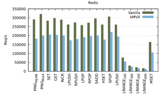
Figure 7: Redis. Geomean overhead of \sim 1.43x for the redis in-memory database using redis-benchmark .
